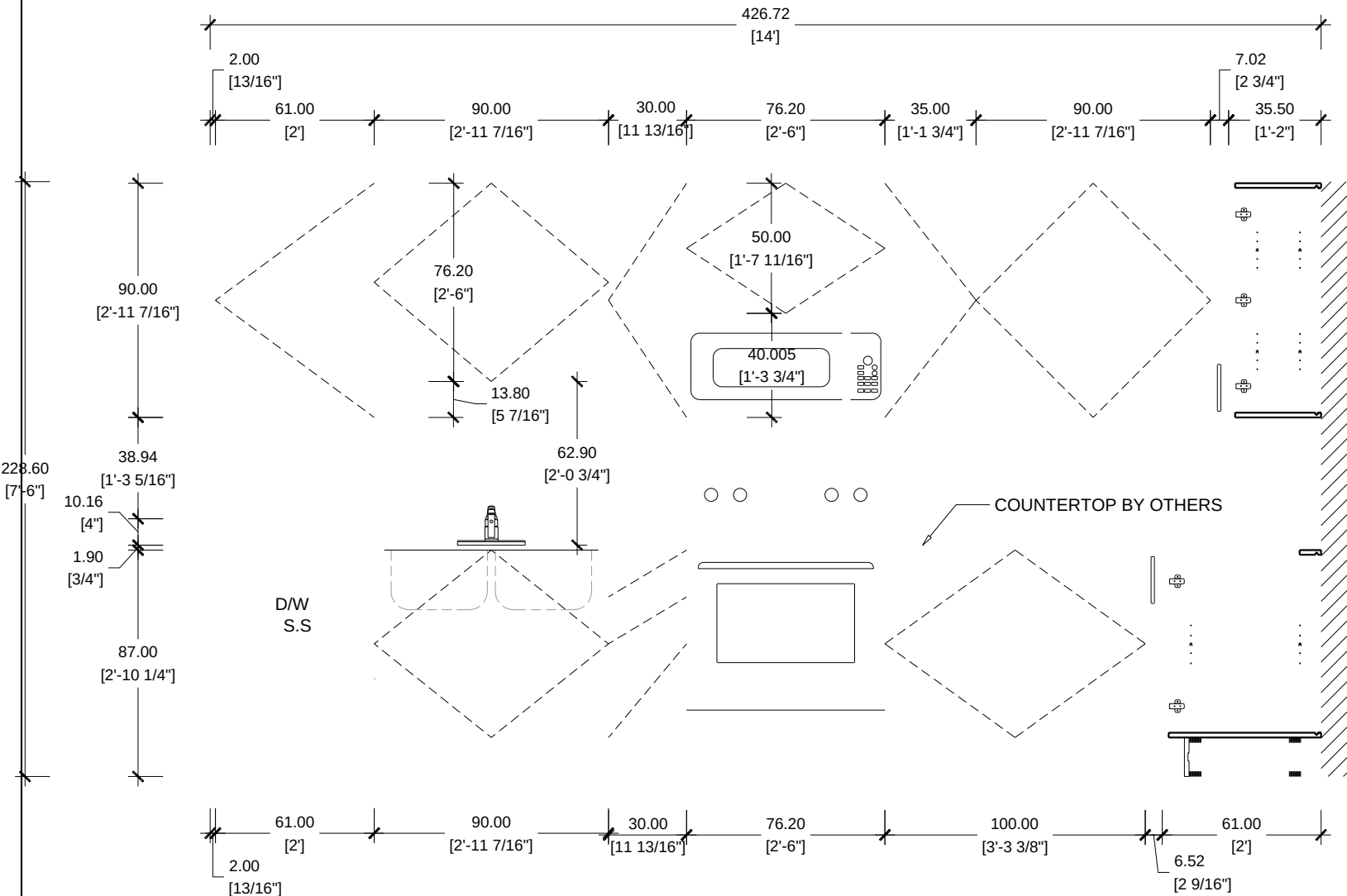
ELEVATION A CASA FAMILIA UNIT A1 / KITCHEN TYPE K1
