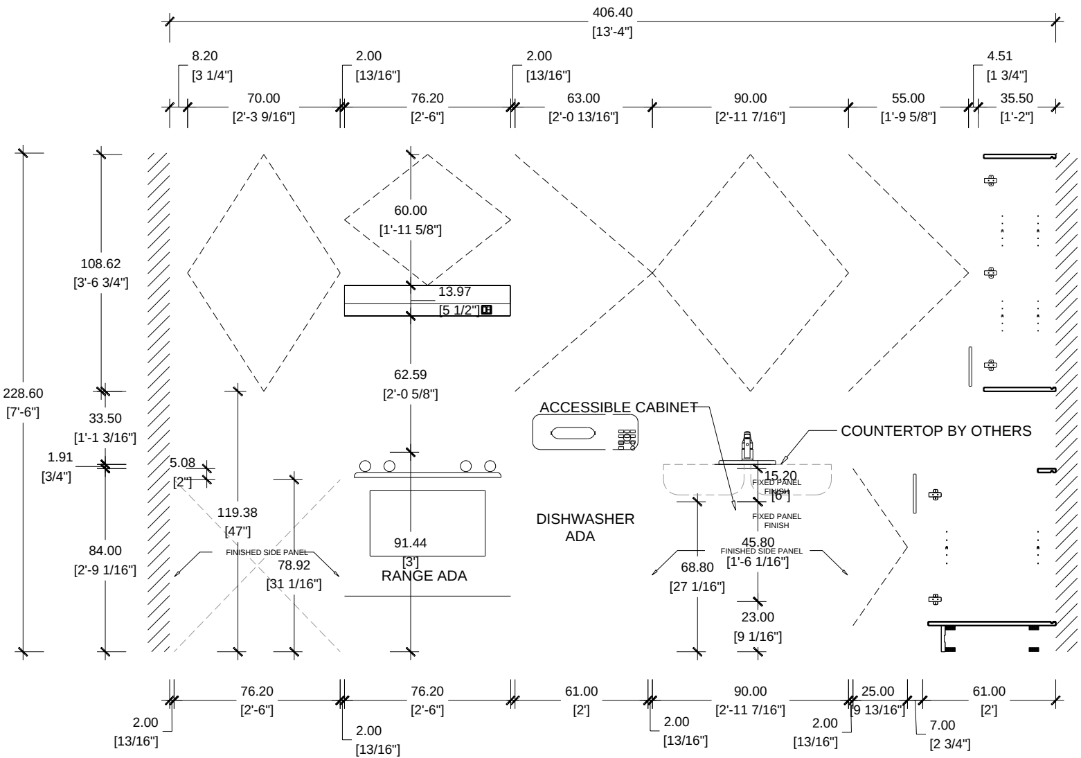
ELEVATION A CASA FAMILIA UNIT B1 FA / KITCHEN TYPE K4 ADA
