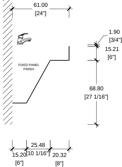
SIDE VIEW SCALE 1/2"=1'-0" CASA FAMILIA / VANITY TYPE RV2
