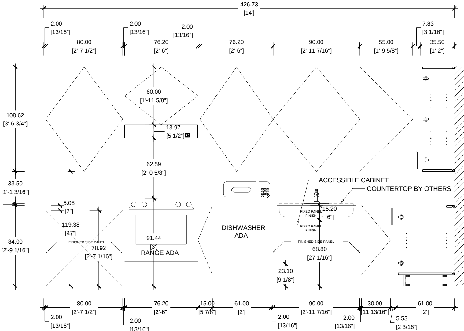
ELEVATION A CASA FAMILIA UNIT A2 FA / KITCHEN TYPE K2 ADA
