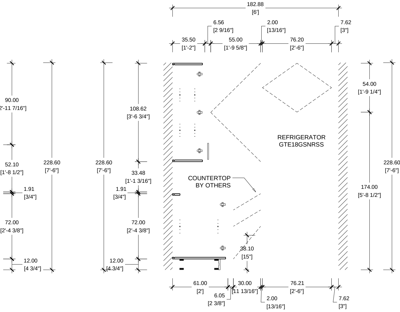
ELEVATION B CASA FAMILIA UNIT A2 FA / KITCHEN TYPE K2 ADA
