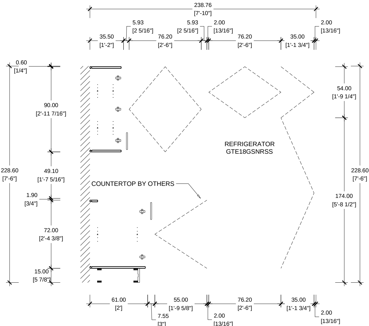
ELEVATION B CASA FAMILIA UNIT A1 / KITCHEN TYPE K1
