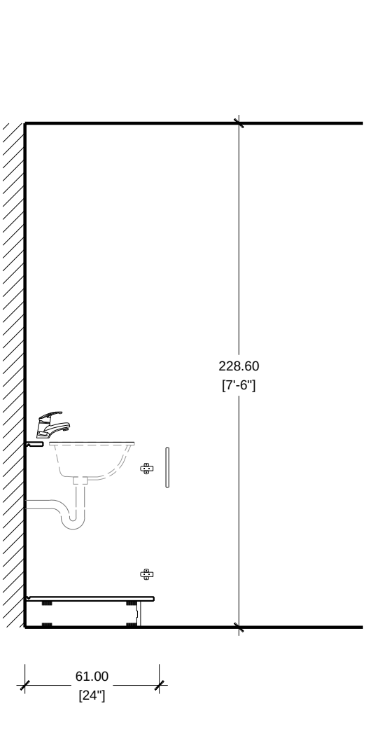
SECTION SCALE 1/2"=1'-0" VANITY
