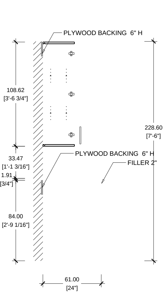
SECTION SCALE 1/2"=1'-0" KITCHEN ADA
