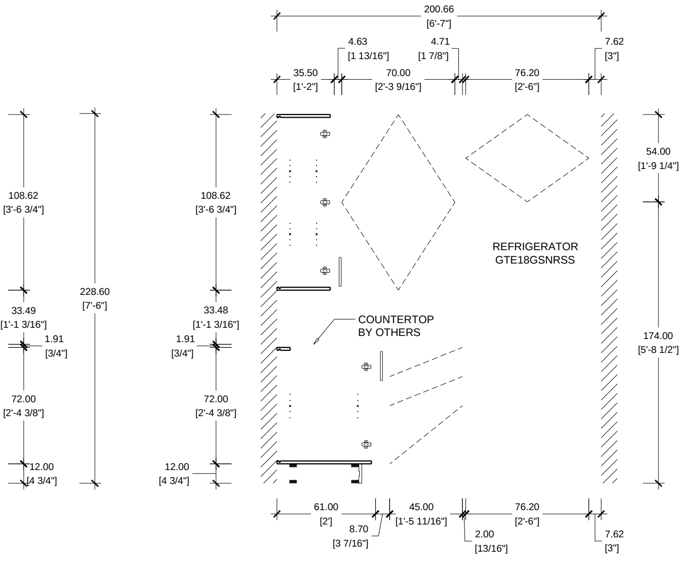
ELEVATION B CASA FAMILIA UNIT B1 FA / KITCHEN TYPE K4 ADA
