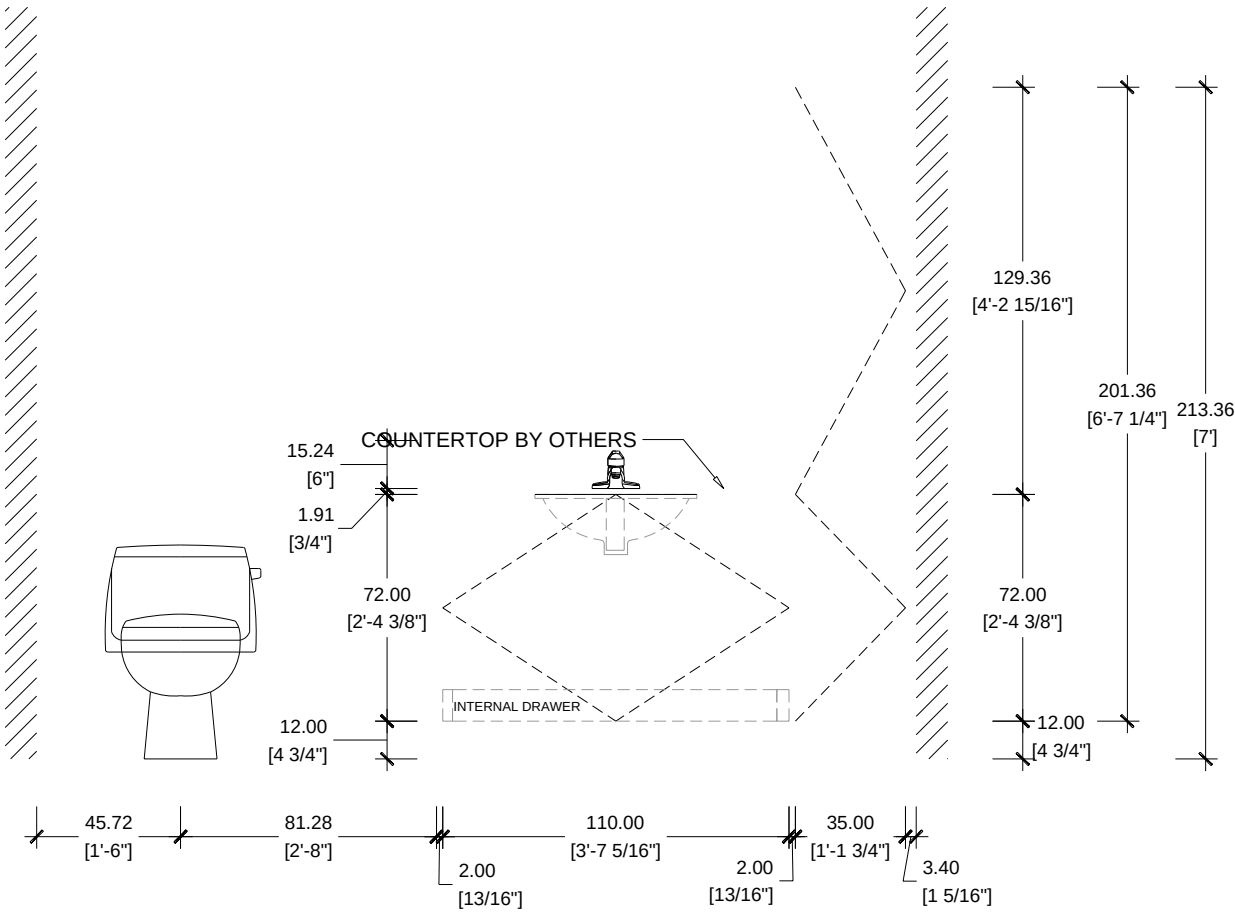
ELEVATION A CASA FAMILIA UNIT B1 / VANITY TYPE V1
