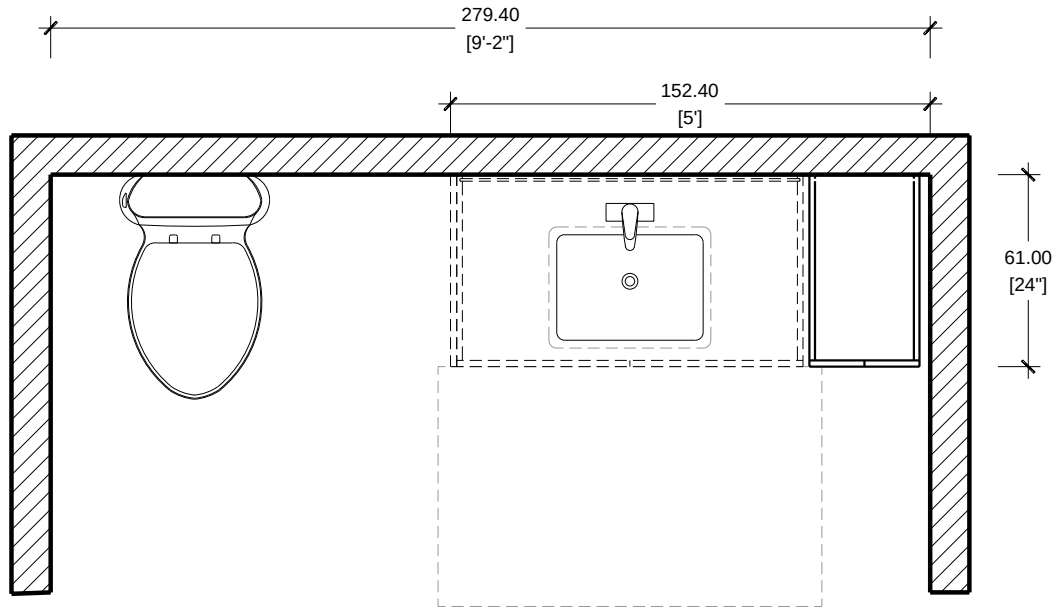
FLOOR PLAN SCALE 1/2"=1'-0" CASA FAMILIA UNIT B1 / VANITY TYPE V1
