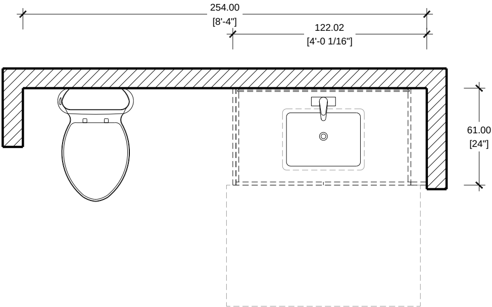
FLOOR PLAN SCALE 1/2"=1'-0" CASA FAMILIA / VANITY TYPE V4
