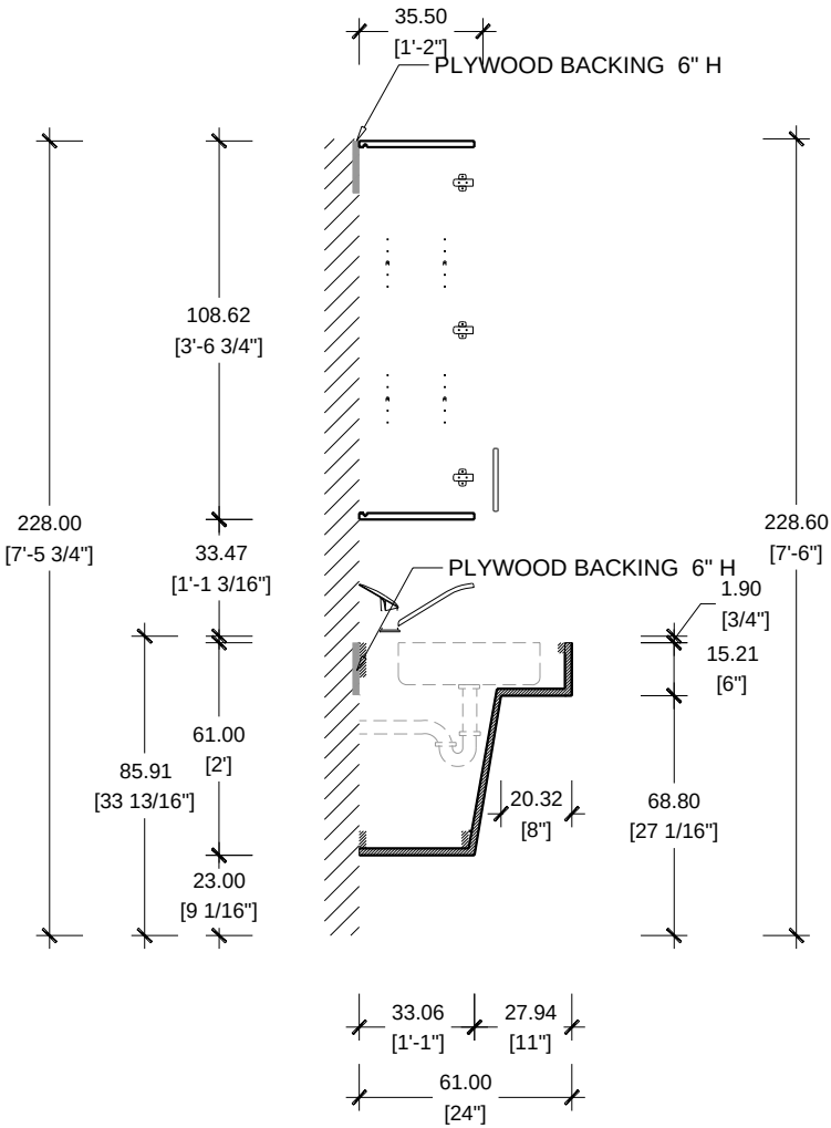
SECTION SCALE 1/2"=1'-0" KITCHEN ADA
