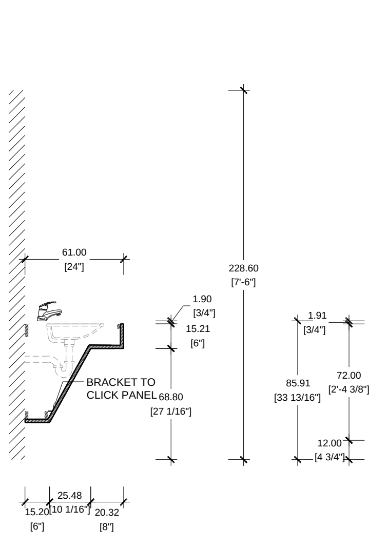
SECTION SCALE 1/2"=1'-0" VANITY ADA
