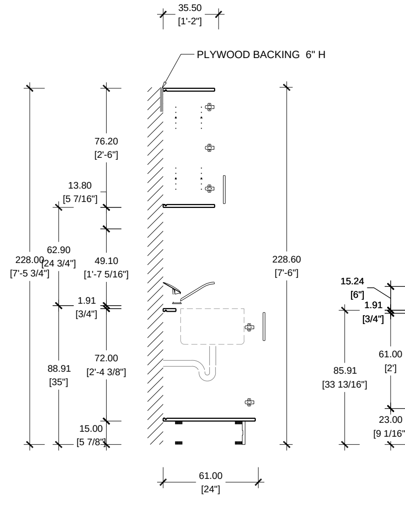
SECTION SCALE 1/2"=1'-0" KITCHEN
